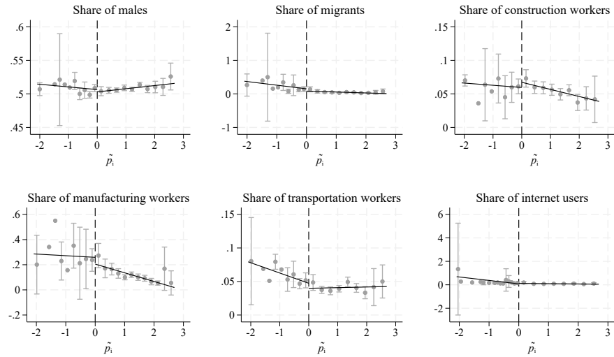
Figure A8. RD Plots of Pre-reform Covariates
