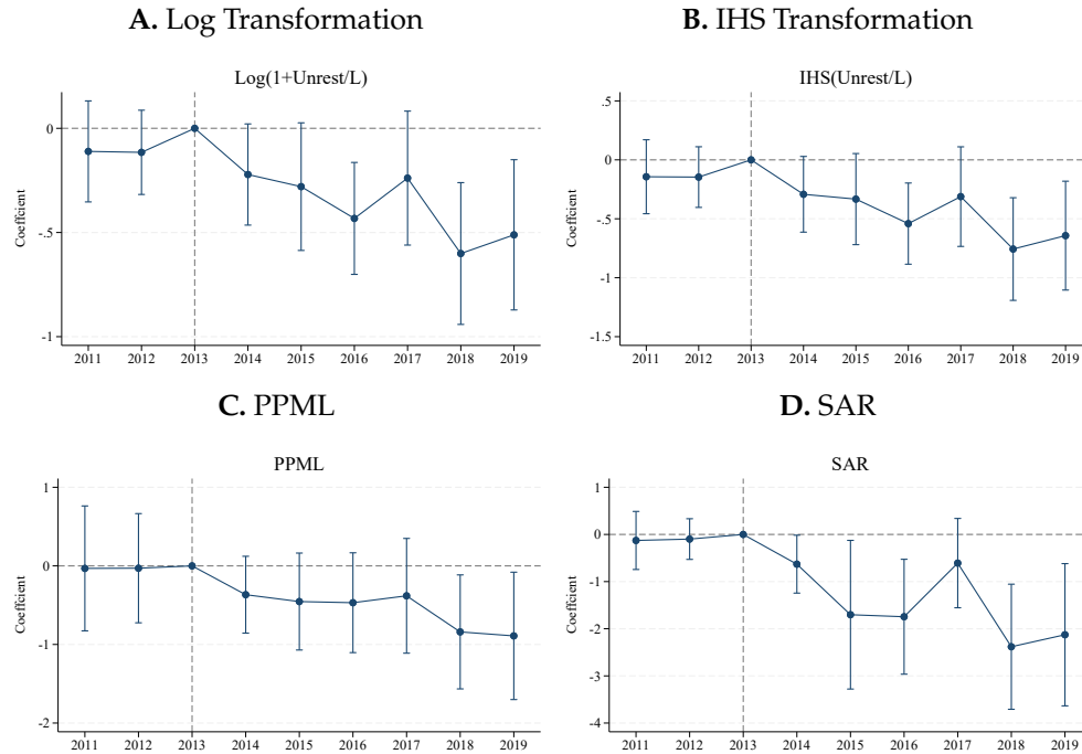
Figure H1. Robustness: Alternative Specifications and Estimators, Event-Study Results
