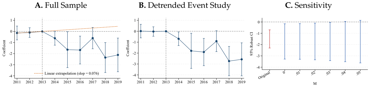
Figure G2. Detrended Event-Study Coefficients and Application of Rambachan and Roth (2023)
