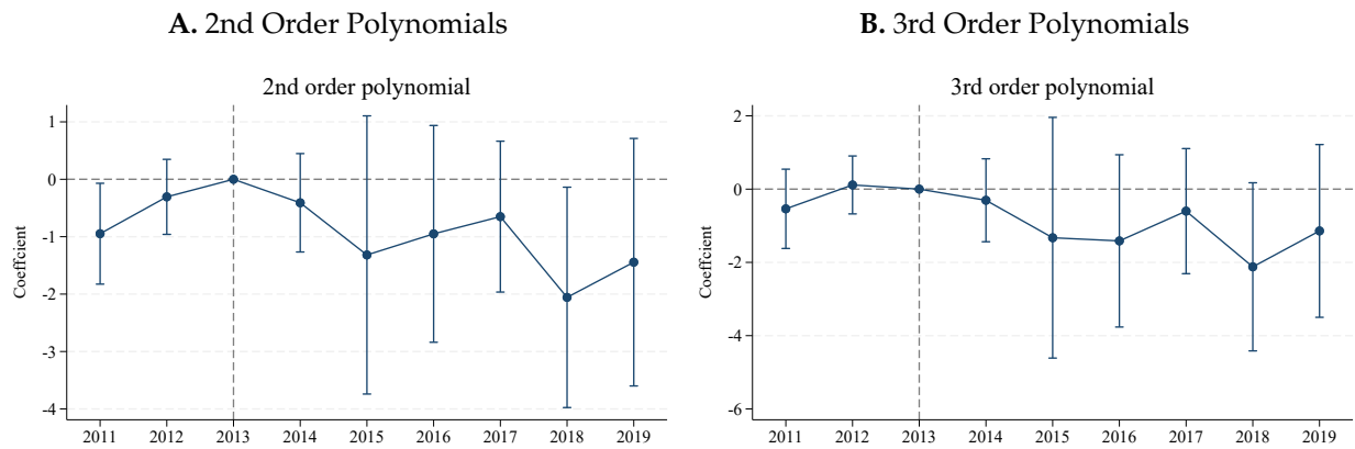
Figure G5. Robustness to Alternative Polynomial Orders
