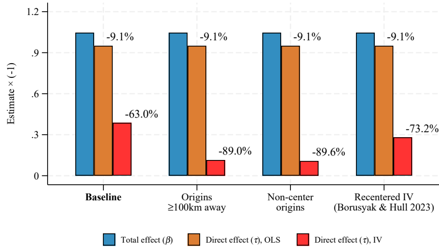
Figure K2. Mediation Visualized: Alternative IVs
