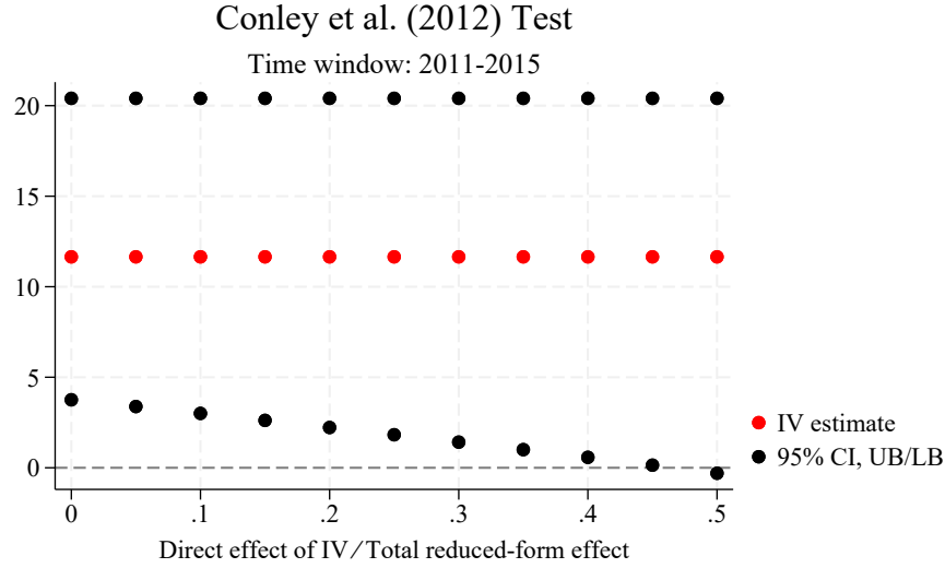
Figure K3. Conley et al. (2012) Test
