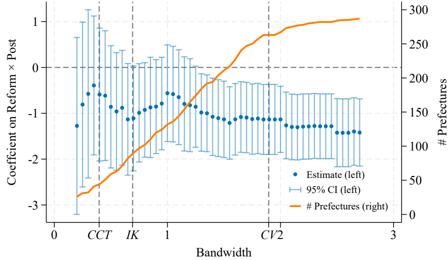
Figure G3. Estimates under Different Bandwidth Choices
