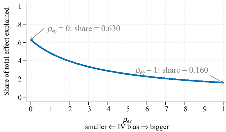
Figure 7. Sensitivity Test for Causal Mediation Analysis
