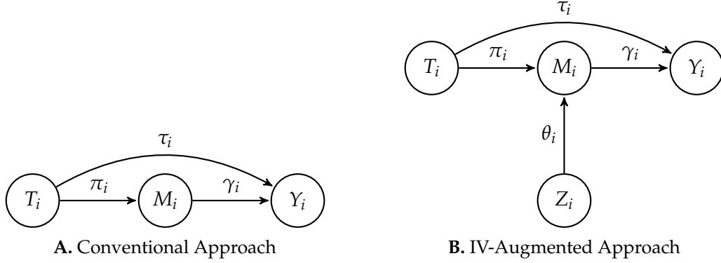
Figure 4. Directed Acyclic Graphs
