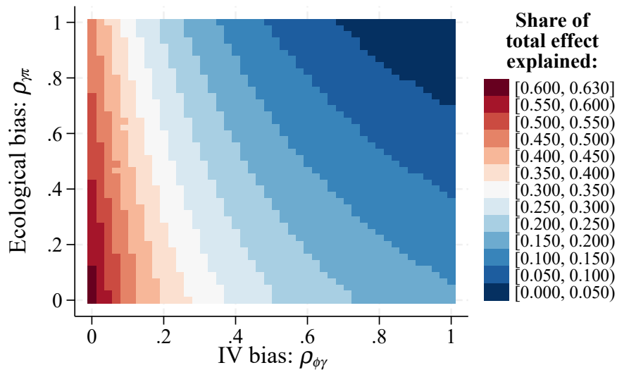
Figure K4. Sensitivity Test for Causal Mediation Under General Framework
